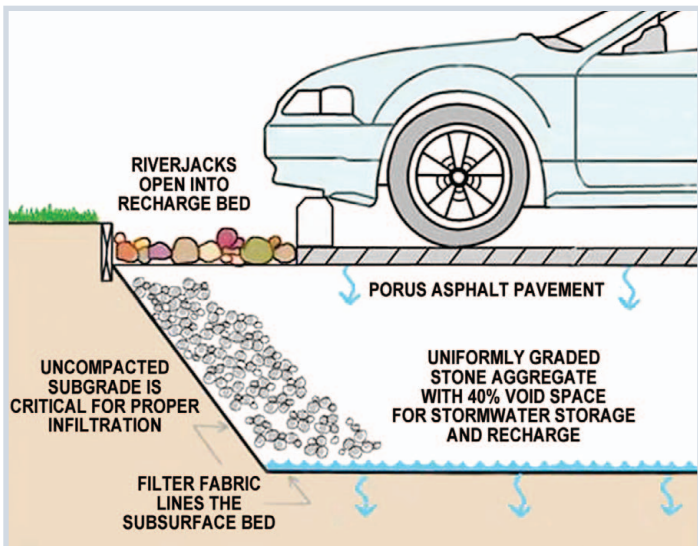
Porous asphalt.
